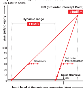
Dynamic range characteristics
