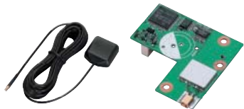
UT-123 D-STAR unit and GPS receiver
